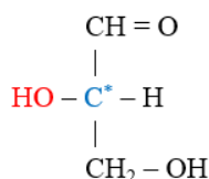
L- glyceraldehyd
