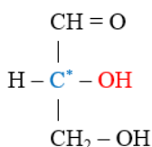
D- glyceraldehyd
